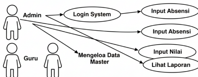
Gambar 2. Use Case Diagram
