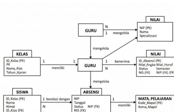
Gambar 4. Entity Relationship Diagram (ERD)
