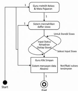
Gambar 3. Activity Diagram
