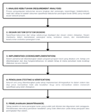
Gambar 1. Proses Metode Waterfall
